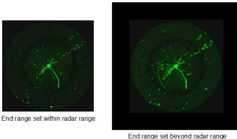
Figure 9: Effect of selecting an end range beyond the radar range
