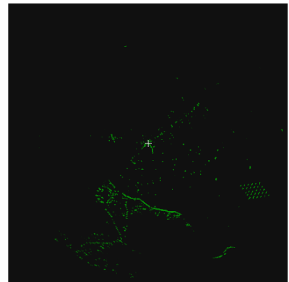
Offset too low. The video intensity is shifted down too far so that small target returns and all of the background noise are below zero intensity and the HPx no longer sees them, resulting in a loss of data.
