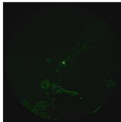
Gain too low. The radar video appears washed-out and even strong returns only give low intensity values.
