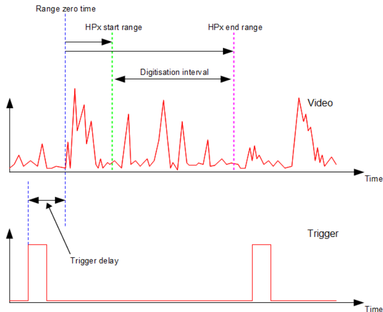
Figure 8: HPx digitisation range settings
