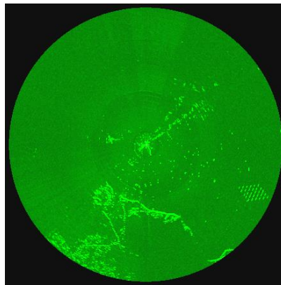
Offset too high. The entire video, including the background noise, is shifted up in intensity. Effectively a DC offset has been applied. The lowest video value will be greater than zero and the highest values will be clipped. This means that the full dynamic range is not being used and the video appears saturated.
