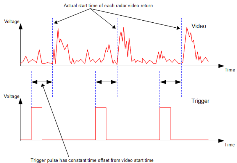
Figure 3: Constant time offset between radar video start range and trigger pulse
