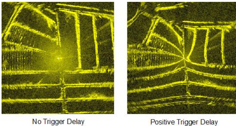
Figure 6: The effect of a positive trigger delay on radar video
