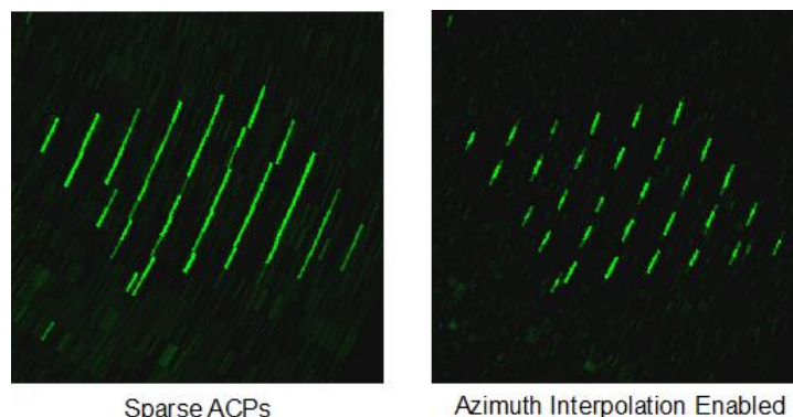
Figure 10: Effect of azimuth interpolation on a radar video display
