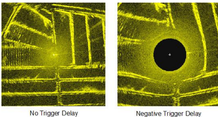
Figure 7: The effect of a negative trigger delay on radar video
