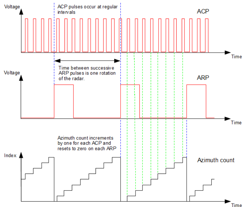
Figure 2: ACP and ARP pulses and the internal azimuth index
