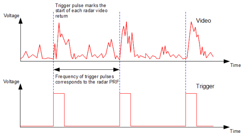
Figure 1: Video signal and corresponding trigger pulses
