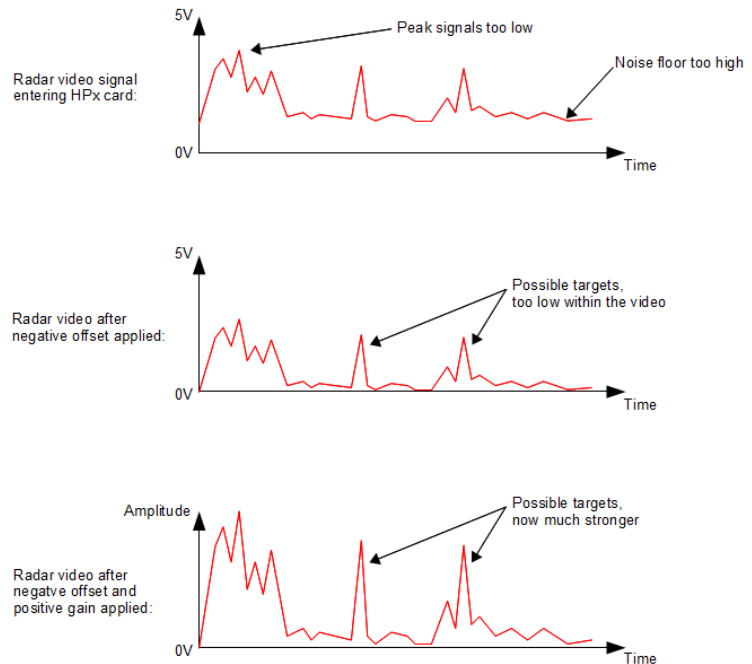
Figure 4: Example of using offset and gain to maximise signal-to-noise ratio
