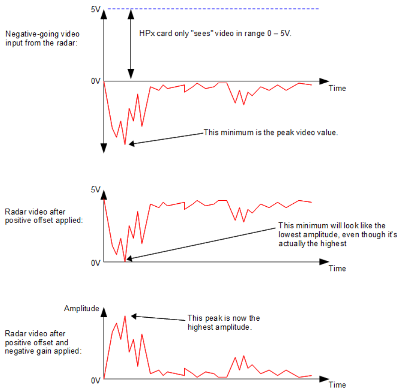
Figure 5: Using gain and offset to compensate for negative-going video
